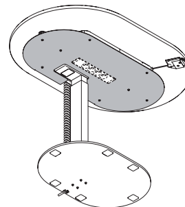
Preparation for connection plug board under the table
