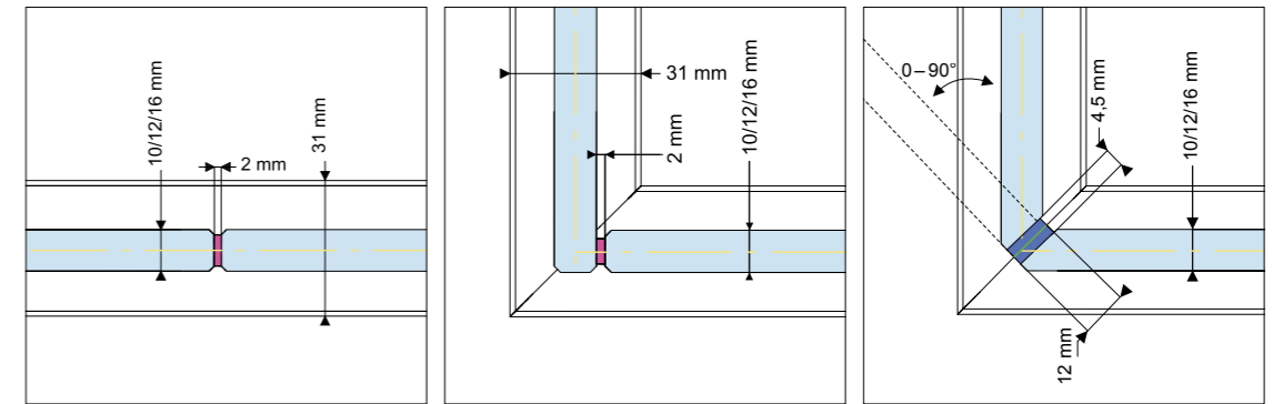
Linear connections
