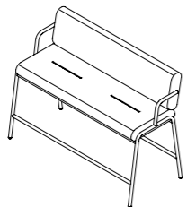
DOUBLE BENCH 1.350 x 605 x 998 mm
