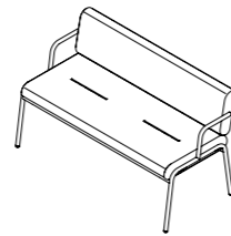
DOUBLE BENCH 1.350 x 655 x 783 mm
